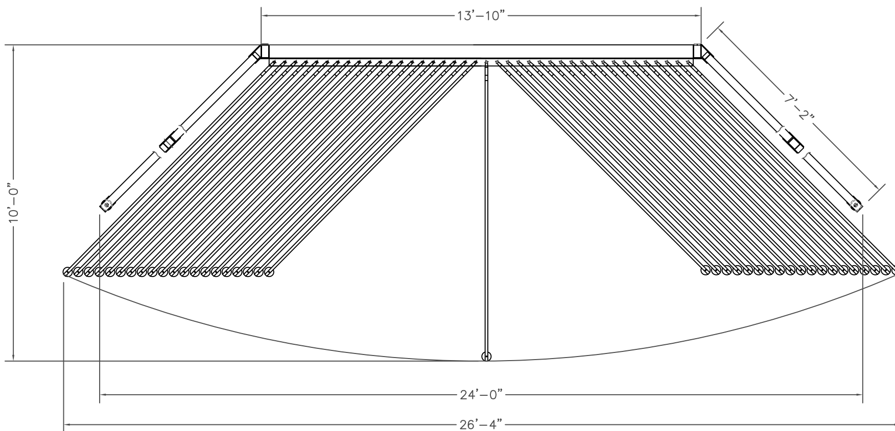
Top View
